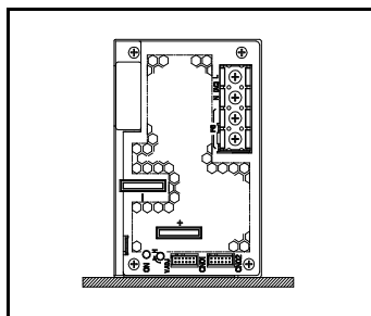
MOUNTING D
