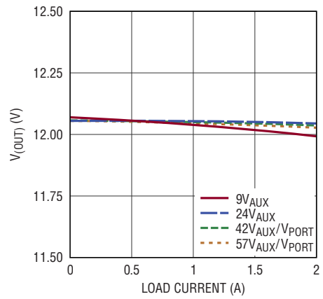
Figure 3. Load Regulation
