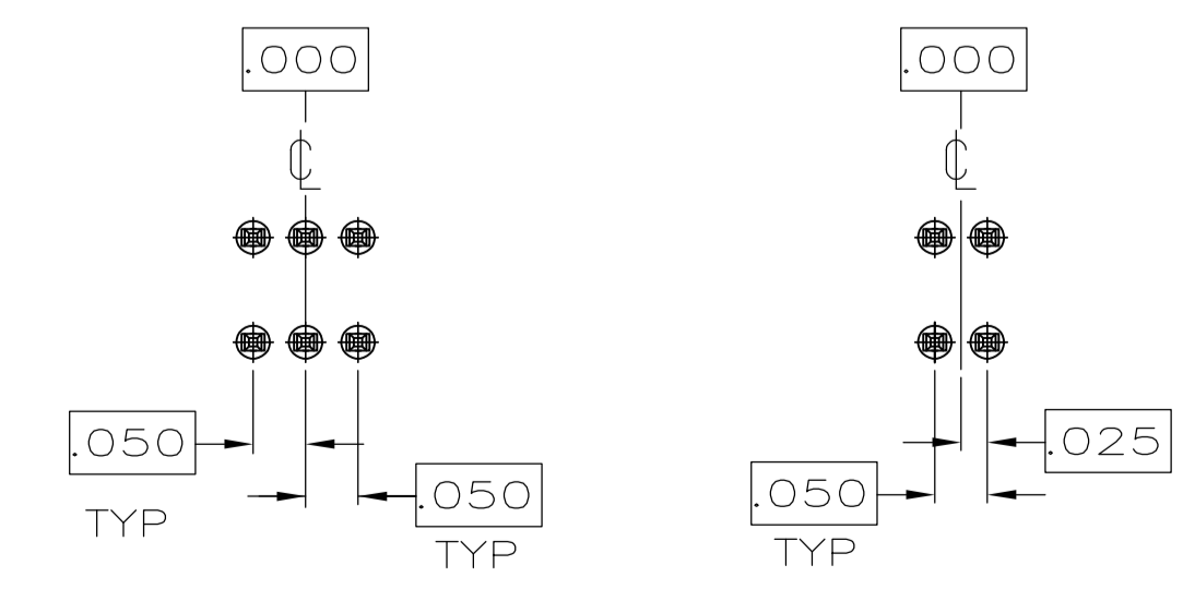
BASIC DIMENSIONS FOR EVEN NO OF SPACES (SEE TABLE) BASIC DIMENSIONS FOR ODD NO OF SPACES (SEE TABLE) DETAIL R
